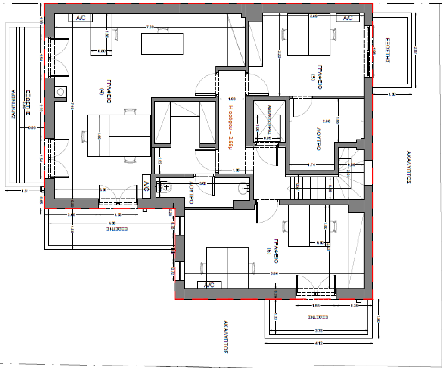
1 st FLOOR
